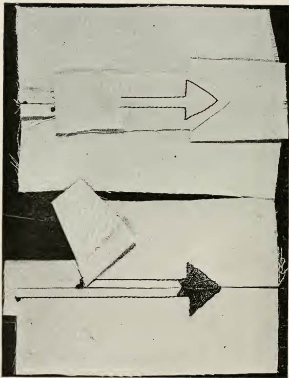
SLOT SEAM FINISHED WITH ARROW HEAD
